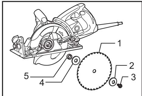
► 1. Saw blade 2. Outer flange 3. Hex bolt 4. Inner flange 5. Ring 17
